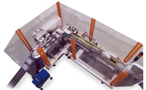
Layout of a typical Right angle 3 Flap Box closer (BC3) (mirror version available)
