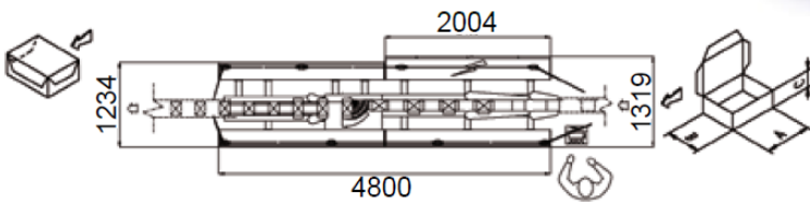
Layout of a typical 3 Flap Box closer (BC3) (mirror version available)
