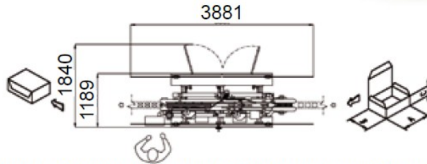
Layout of a typical 1 Flap Box closer (BC1) (mirror version available)
