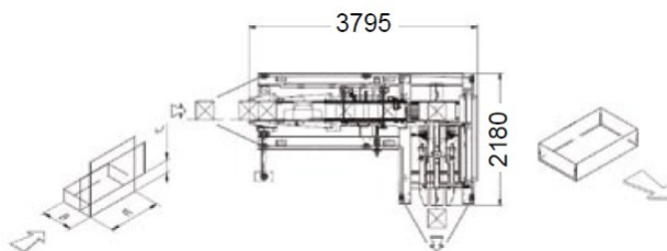
Layout of a typical Right angle 3 Flap Box closer (BC3) (mirror version available)
